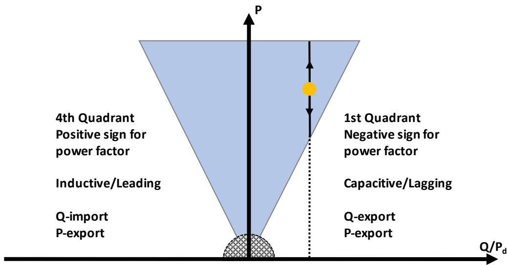
Figure 5.13 – Example of Q control [Q set point].
