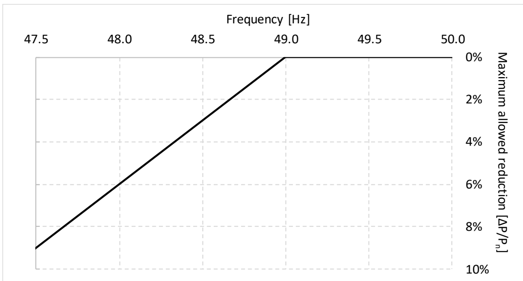
Figure 5.2 – Permitted reduction of active power during underfrequency.
