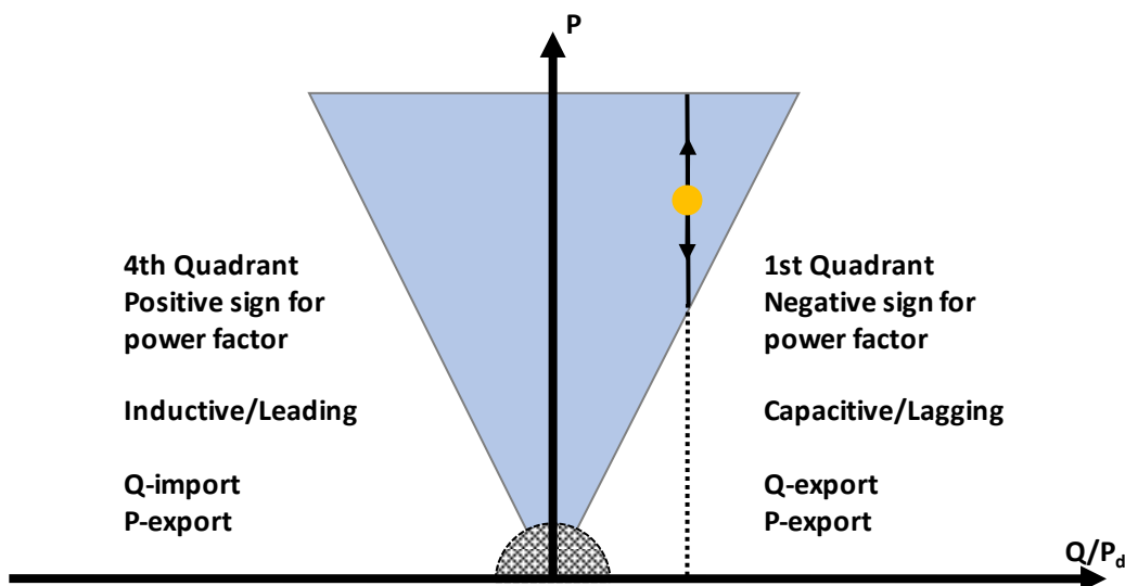
Figure 4.10 – Example of Q control [Q set point].
